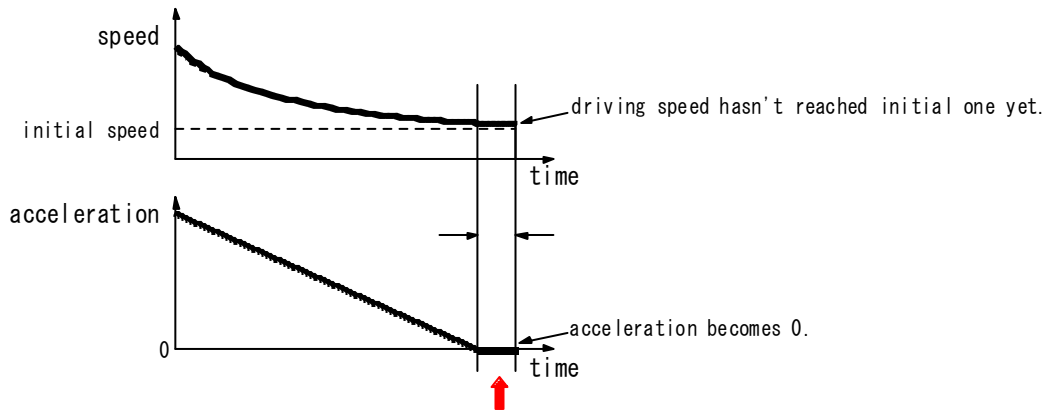
Figure 2. Driving speed and acceleration just before driving completion
