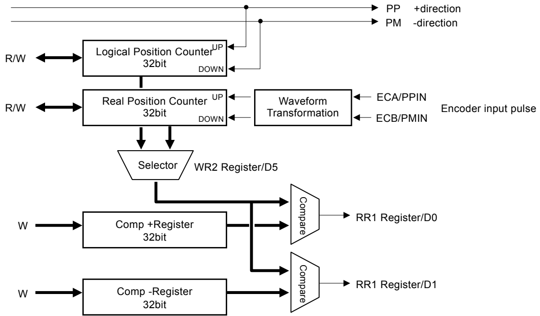
Fig. 2.19 Position Control Block Diagram
