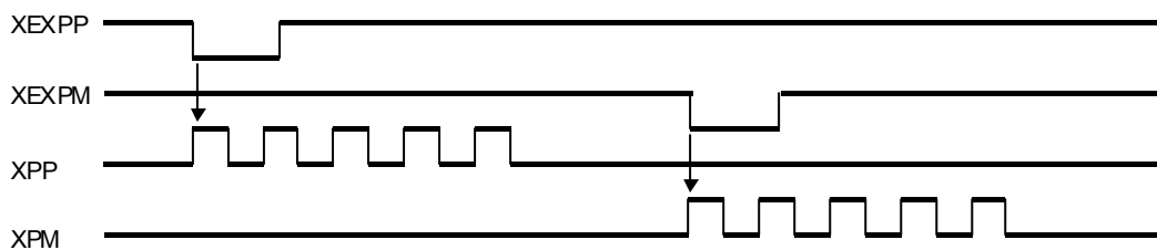
Fig. 2. 26 Example of The Constant Driving by External Signal
