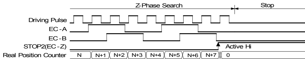
Fig. 2.23 Example of Operation of Clearing The Real Position Counter Using The STOP2 Signal
