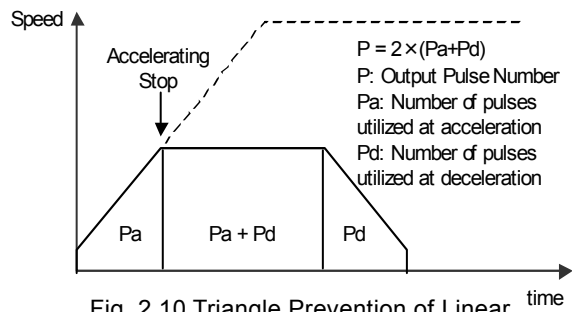
Fig. 2.10 Triangle Prevention of Linear Acceleration Driving
