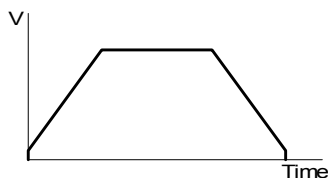
Trapezoidal Acceleration/Deceleration Driving (Symmetry)
