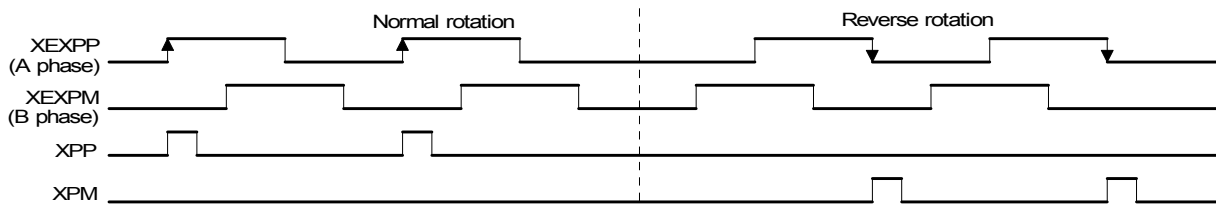
Fig. 2.28 Example Output Pulse 1 Driving by A Manual Pulsar
