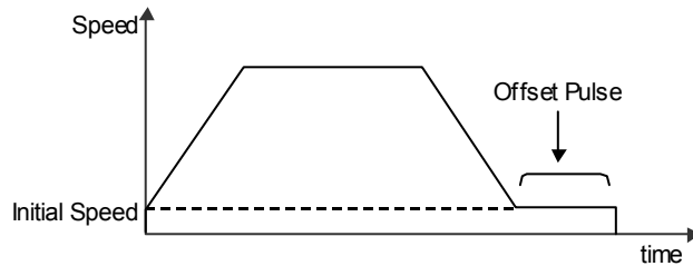
Fig.2.6 Offset for Deceleration
