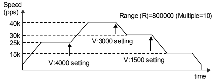
Fig.2.5 Example of Drive Speed Change During Driving
