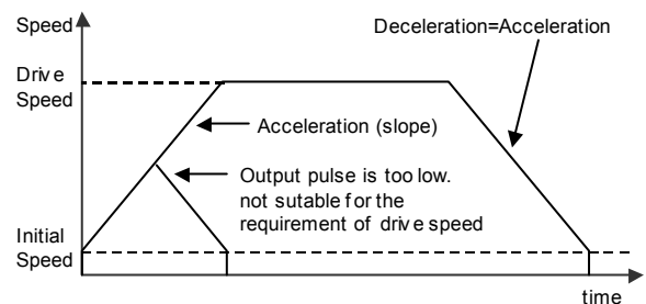
Fig. 2.9 Trapezoidal Driving (Symmetrical)
