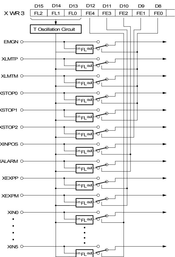
Fig. 2.44 Concept of Input Signal Filter Circuit
