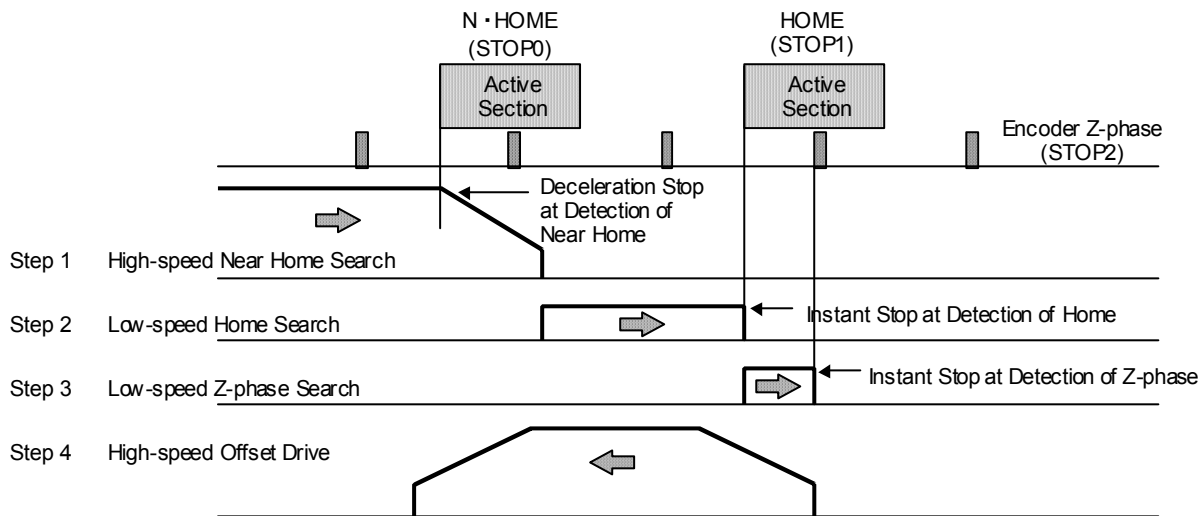
Fig. 2.24 Prototype of Automatic Home Search Using This IC
