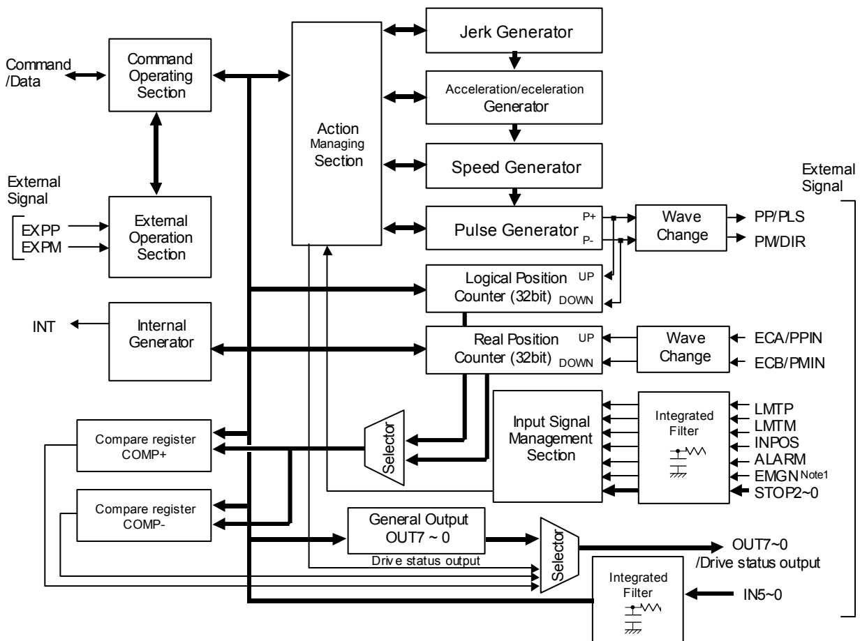
Fig. 1-1 MCX302 Functional Block Diagram
