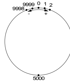
Fig. 2.21 Operation of Position Counter Ring Maximum Value 9999
