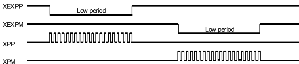
Fig. 2. 27 Example of The Continuous Driving by External Signal
