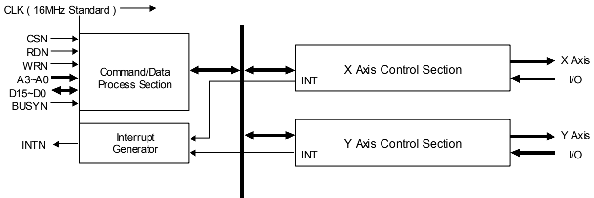
Fig. 1-1 MCX302 Functional Block Diagram
