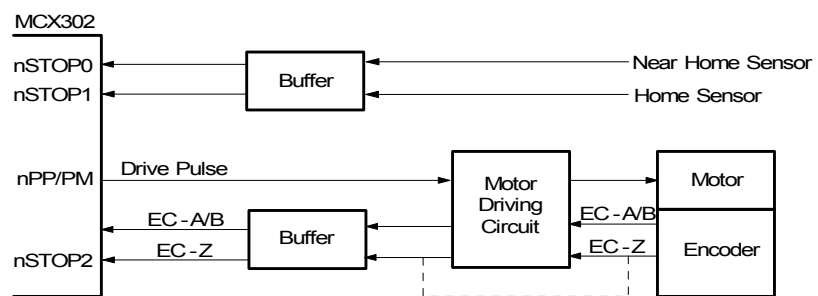
Fig. 2.22 Example of Signal Connection for Clearing The Real Position Counter by The STOP2 Signal
