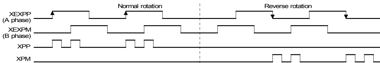
Fig. 2.29 Example of Output Pulse 2 Driving by A Manual Pulsar
